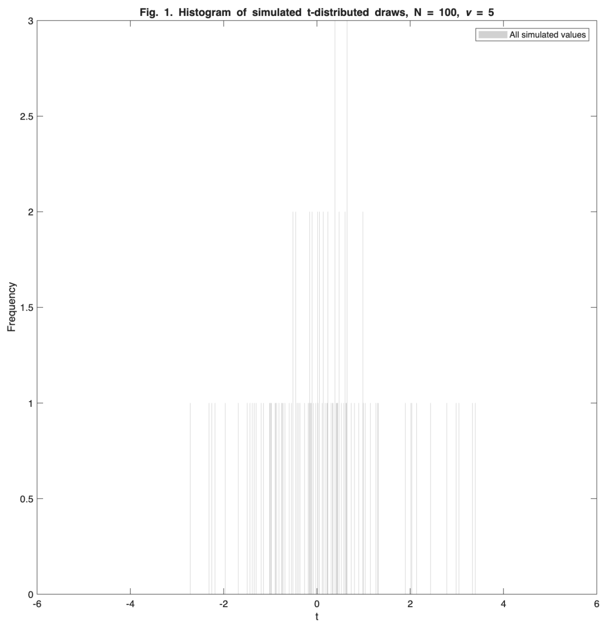
Figure 1: Frequency distribution of 100 draws
