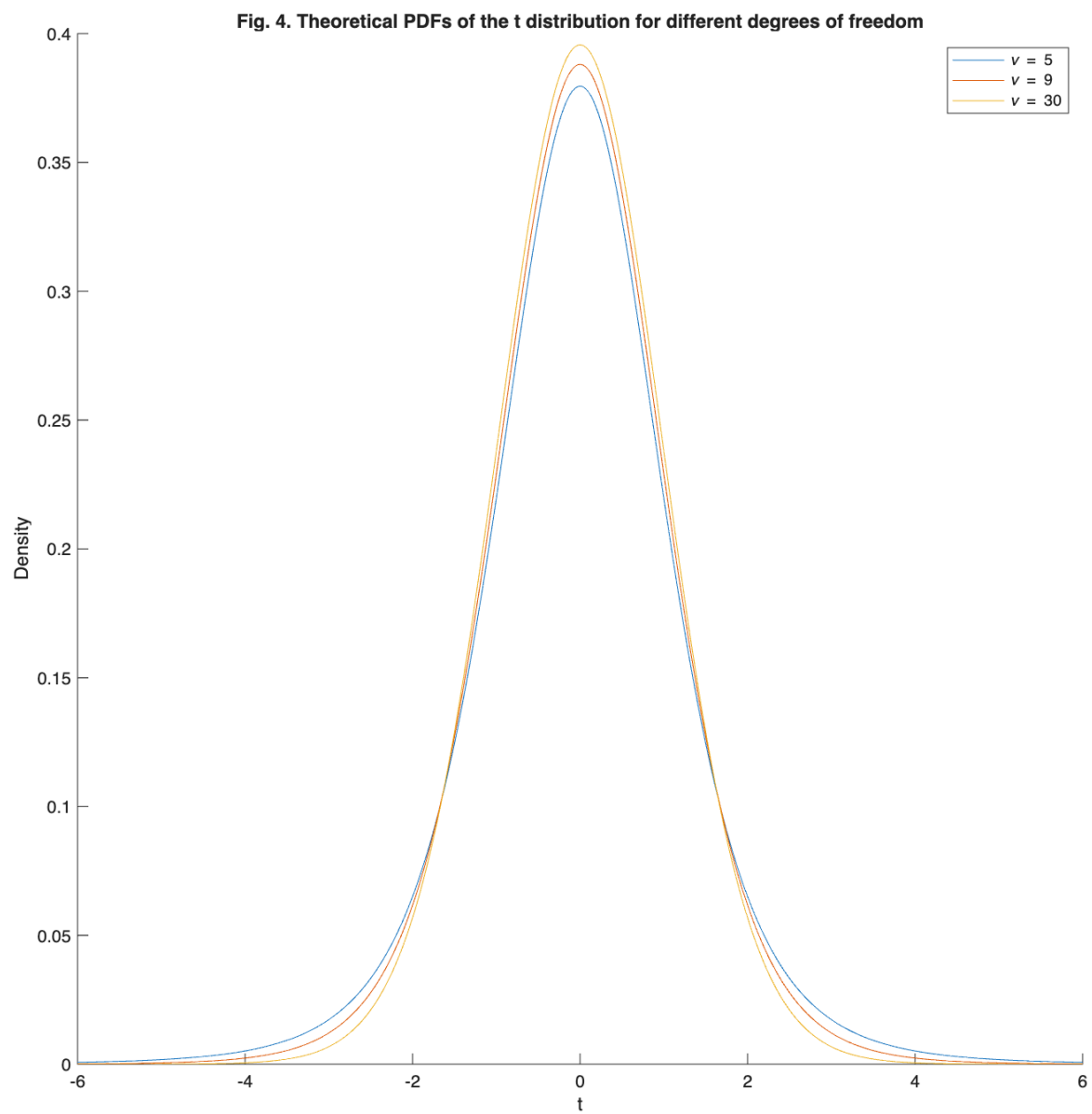
Figure 4: Limiting distributions with different degrees of freedom
