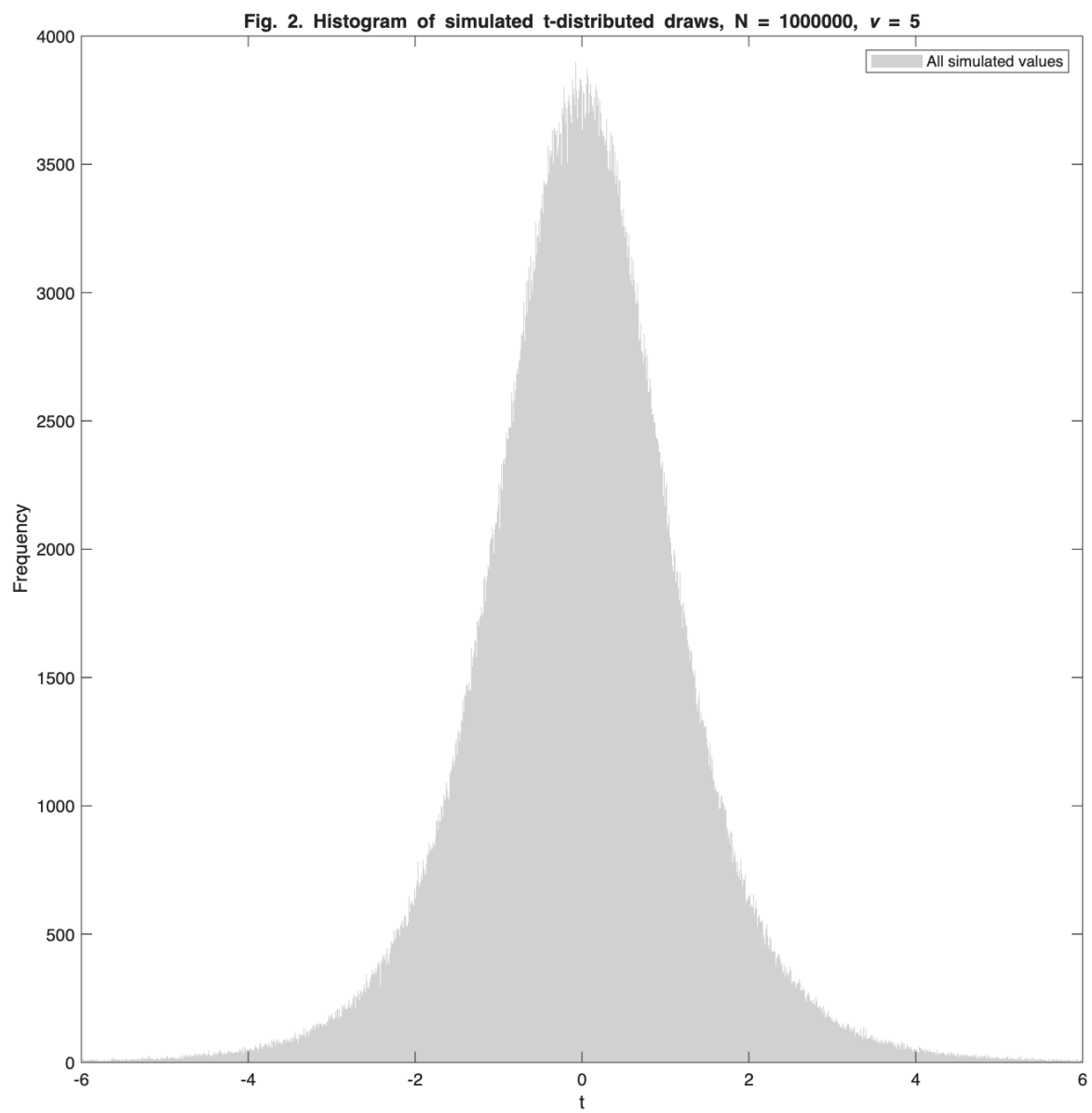
Figure 2: Frequency distribution of 1000000 draws
