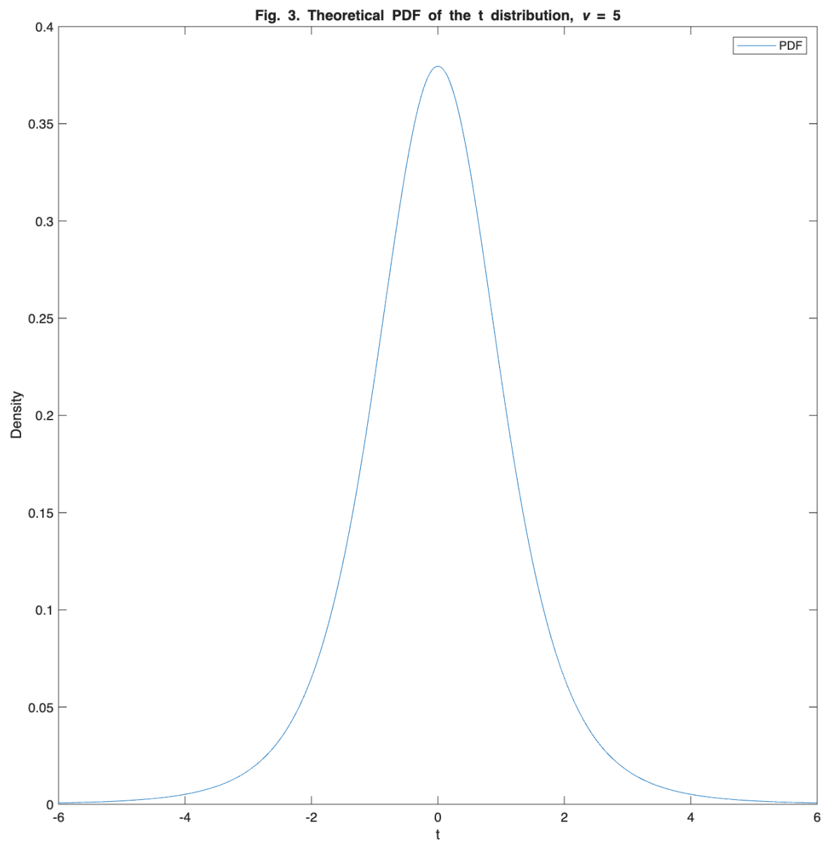
Figure 3: The limiting distribution
